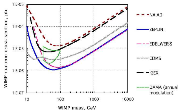
Figure 2: Preliminary limits on WIMP-nucleon spin-independent cross-section from the NAIAD and ZEPLIN I experiments are shown together with some other limits and with a region of parameter space consistent with the DAMA signal (see 1 for recent limits).
